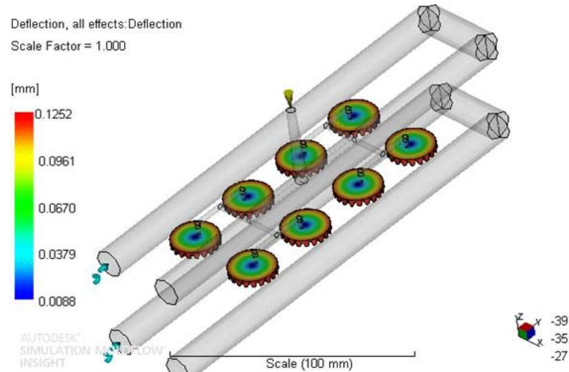
Fig.3 Warpage analysis result of one of the simulation
