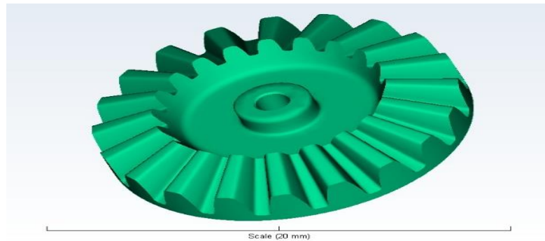
Fig.1 Bevel gear model
