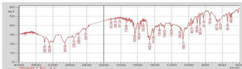
Fig.3 FTIR spectra of Ambroxol hydrochloride and Ethyl cellulose
