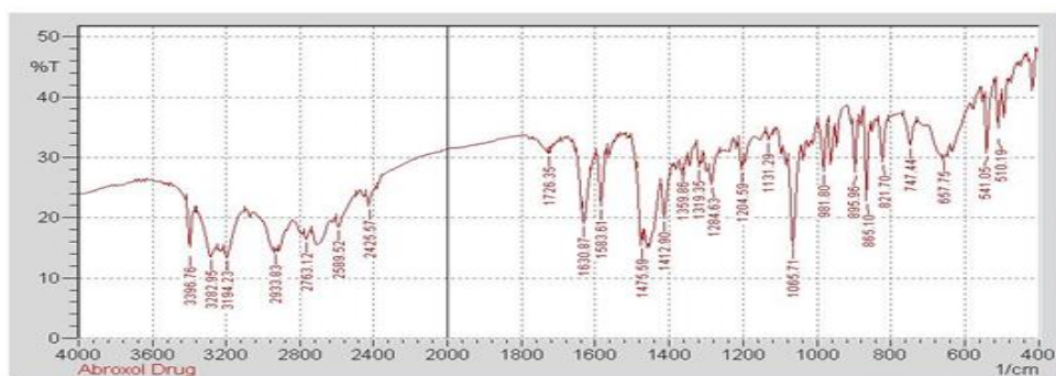
Fig 1.FTIR spectra of Ambroxol Hydrochloride
