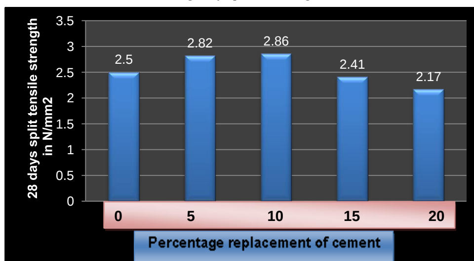
Fig. 28 days split tensile strength
