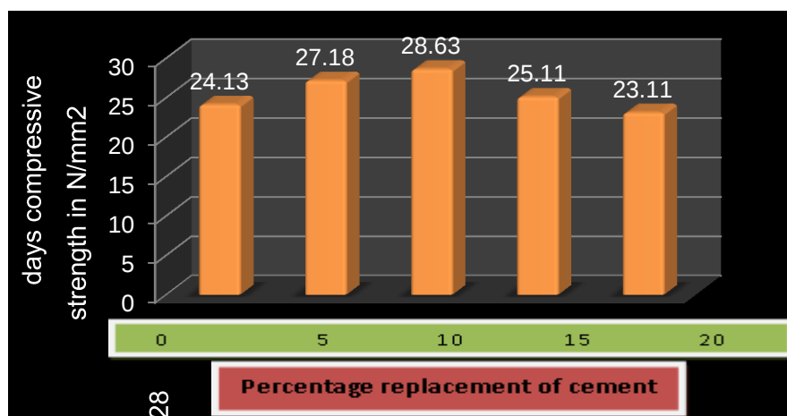
Fig. 7 Days compressive strength
