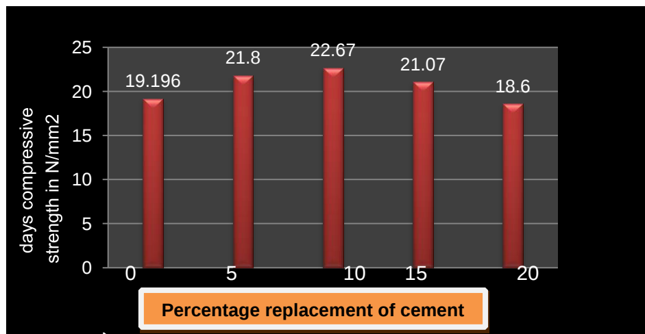
Fig. 7 Days compressive strength
