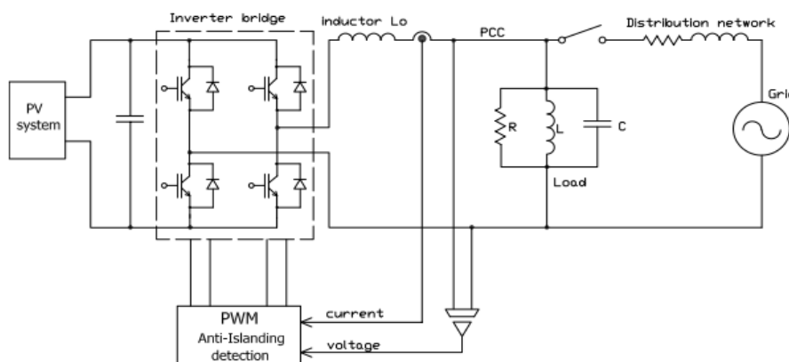
Fig.2 Test system with DG
