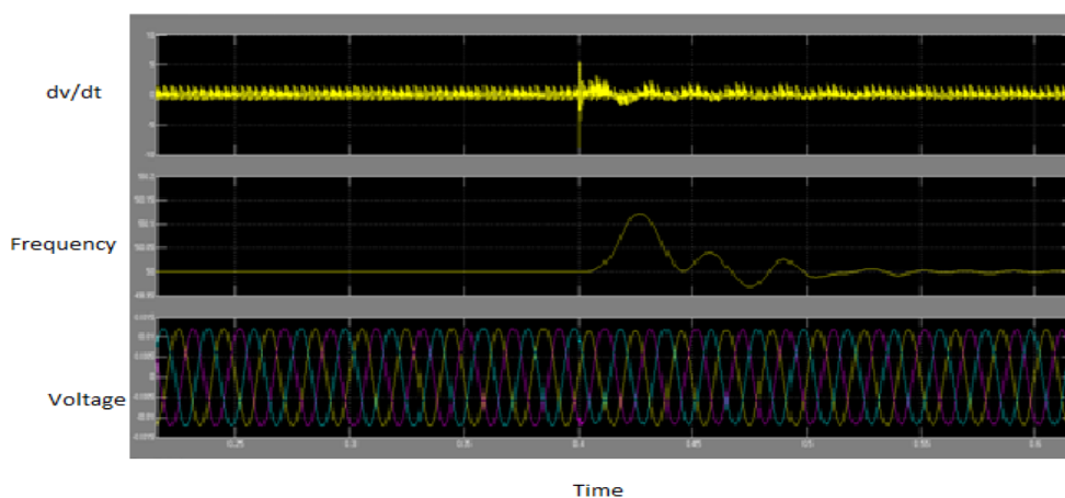
Fig. 5 a) Rate of change of voltage b) System frequency c) System voltage
