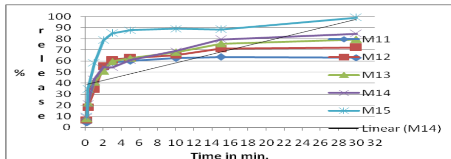
Fig. 6 Drug release profile
