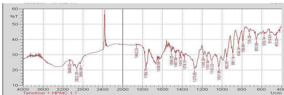
Fig. 4 FTIR spectra of TDF with HPMC E15
