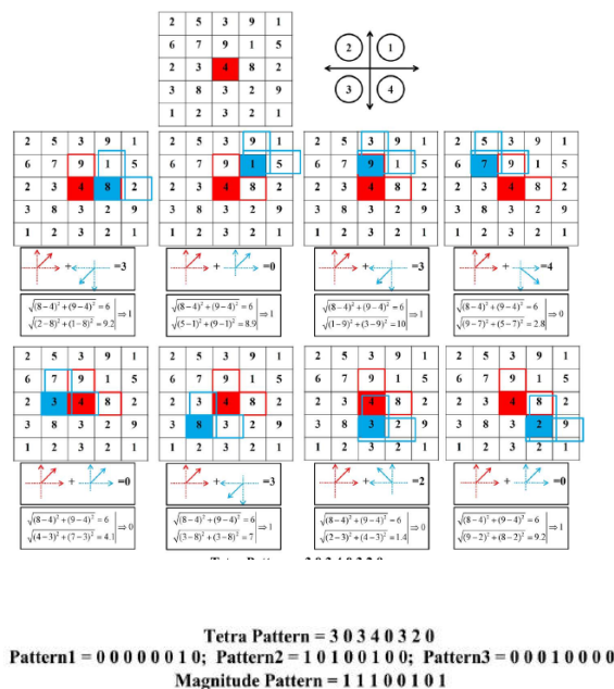
Fig. 3. Example to obtain the tetra and magnitude patterns. For generating a tetra pattern, the bit is coded with the direction of neighbor when the direction of the center pixel and its neighbor are different, otherwise “0.” For the magnitude pattern, the bit is coded with “1” when the magnitude of the center pixel is less than the magnitude of its neighbor, otherwise “0.”
