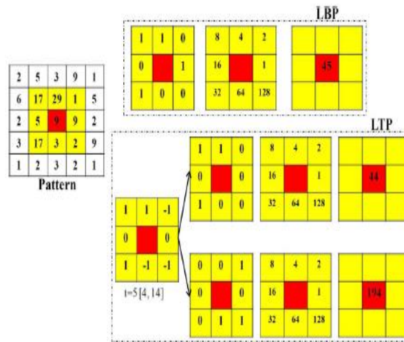
Fig. 1. Calculation of the LBP and LTP operators.
