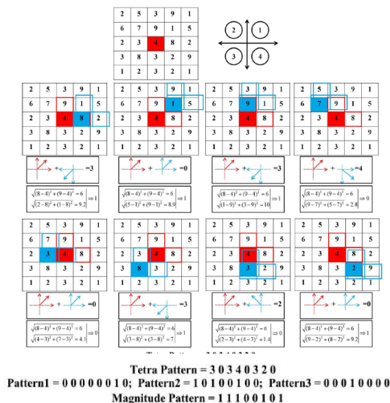
Fig. 3. Example to obtain the tetra and magnitude patterns.
