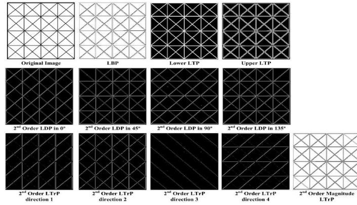
Fig. 4. Each pixel of the original image is considered as the center pixel, and it is coded by using the LBP, LTP, LDP, and LTrP descriptors with the help of neighbors.
