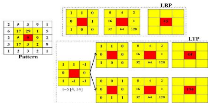
Fig. 1. Calculation of the LBP and LTP operators.
