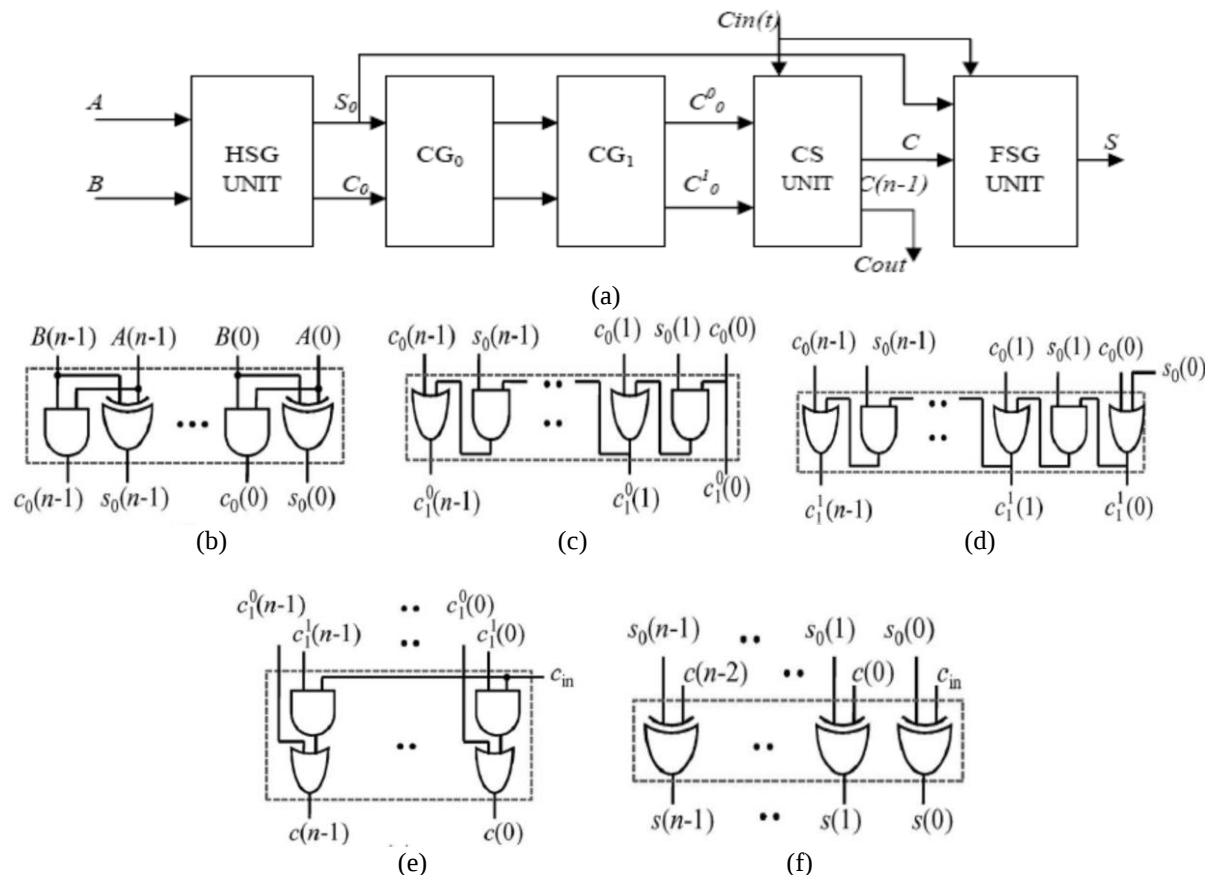
Fig. 3. (a) Proposed CS adder design, where n is the input operand bit-width. (b) Gate-level design of the HSG. (c) Gate-level optimized design of ( CG_0 ) for input-carry = 0. (d) Gate-level optimized design of ( CG_1 ) for input-carry = 1. (e) Gate-level design of the CS unit. (f) Gate-level design of the final-sum generation (FSG) unit.
