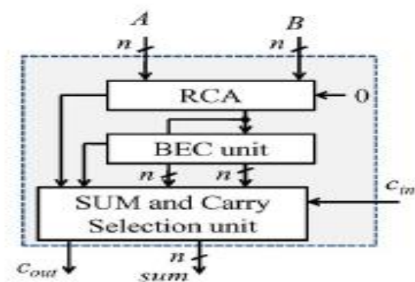
Fig.2 Structure of the BEC-based CSLA; n is the input operand bit-width.
