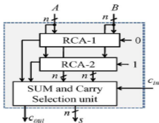
Fig.1 (a) Conventional CSLA; n is the input operand bit-width.
