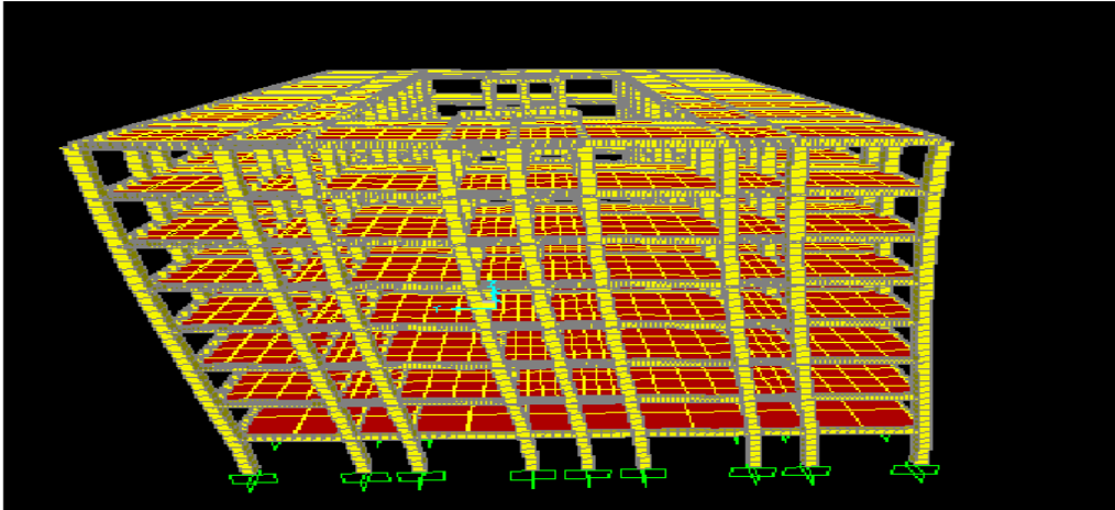
Fig. 7: Deformed shape of bare frame model.
