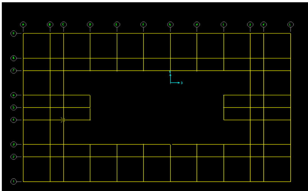
Fig.2 Floor Plan of the building
