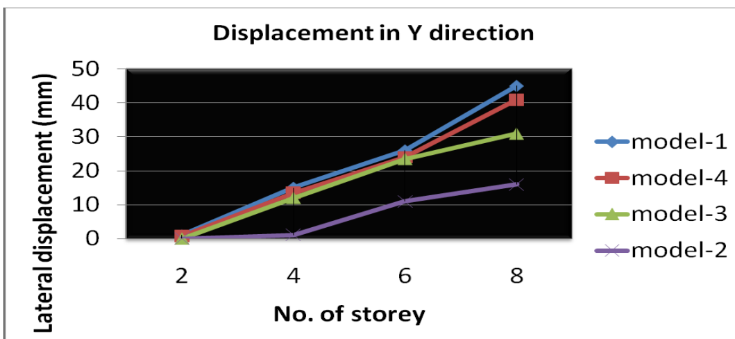
Fig.11 Model Displacements in zone II
