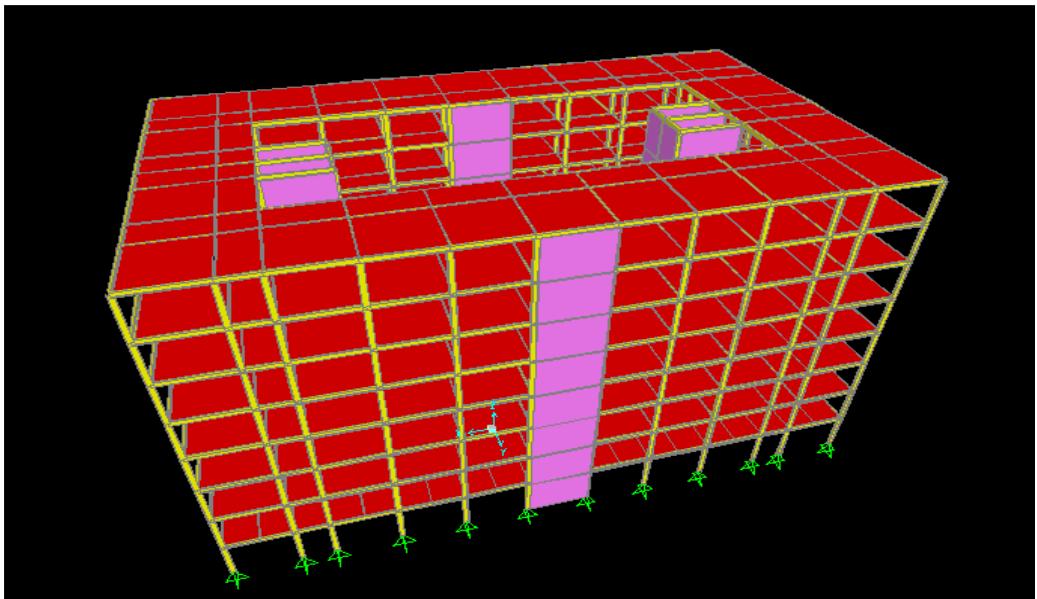
Fig.5 3D Model-3
