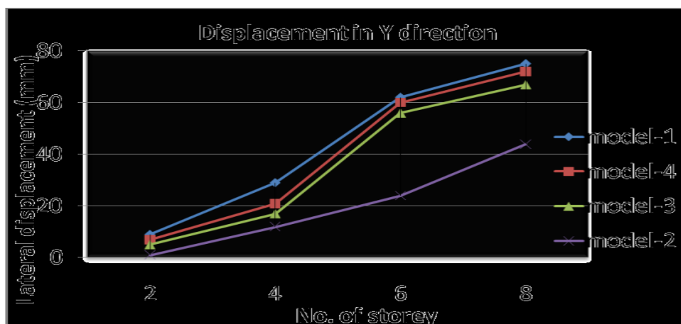
Fig. 9: Model Displacements in zone IV
