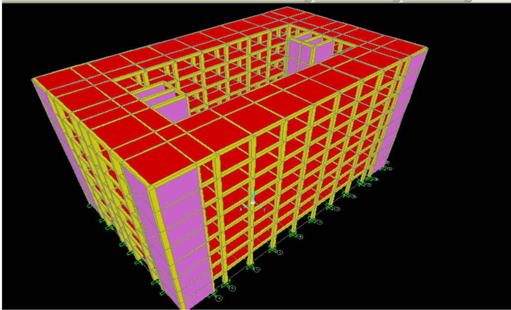
Fig.4 3D Model-2
