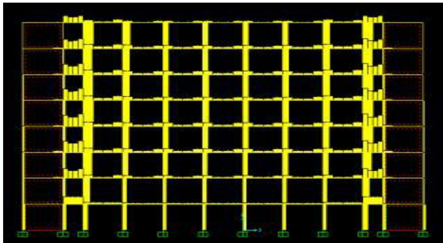
Fig.13 Shear force diagram.
