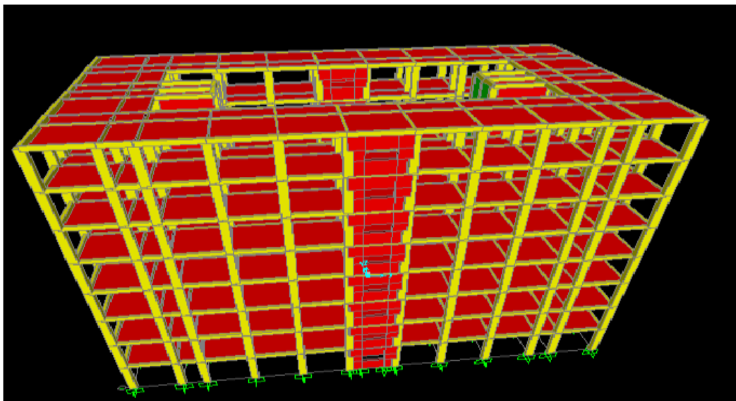
Fig.6 3D Model-4
