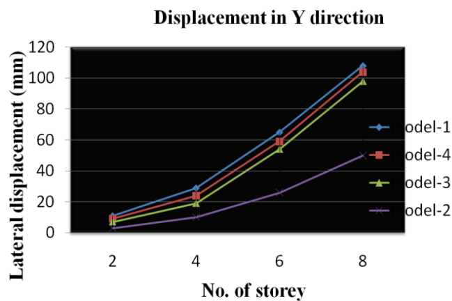
Fig.8 Model displacement in zone V
