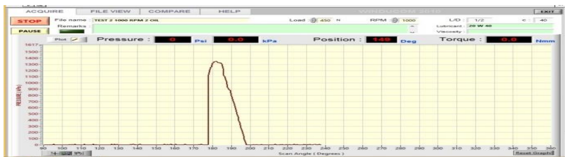
Fig.8 Variation of pressure with angular position and load condition at 1000 rpm and 450N Load Grade Oil SAE 20W40
