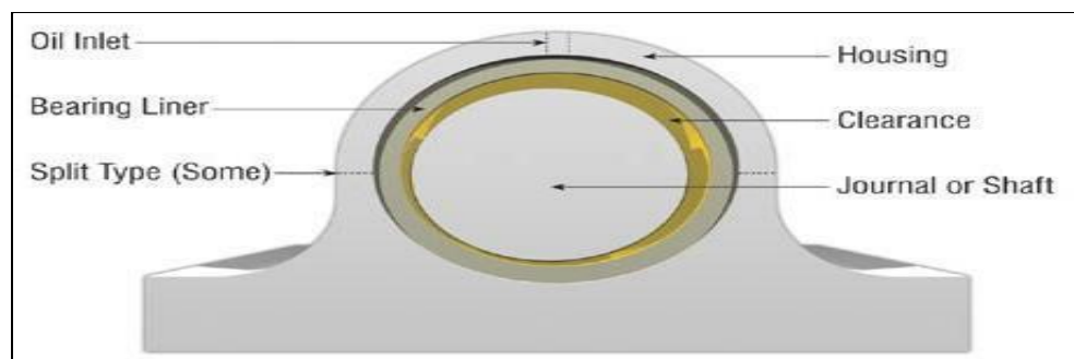
Fig.1 Different components of journal bearing
