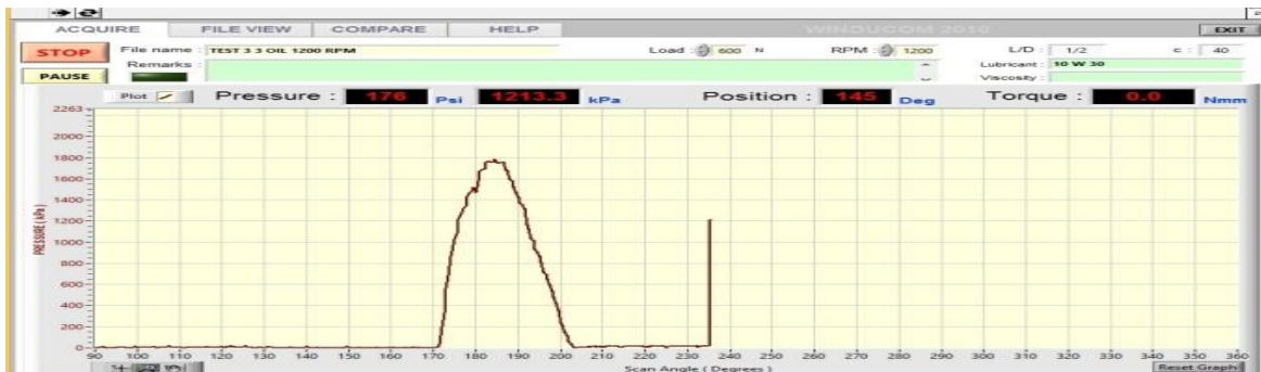
Fig.4 Variation of pressure with angular position and load condition at 1200 rpm and 600 N Load Grade Oil SAE 10W30
