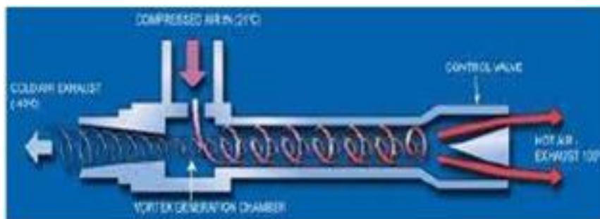
Fig. 4 Schematic diagram of flow pattern in vortex tube
