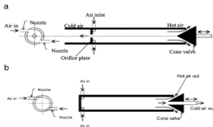
Fig.2 a counter-flow vortex tube b. uni-flow vortex tube
