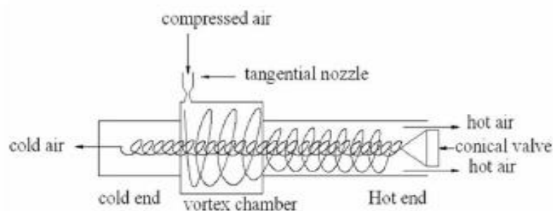
Fig.1 Vortex Tube
