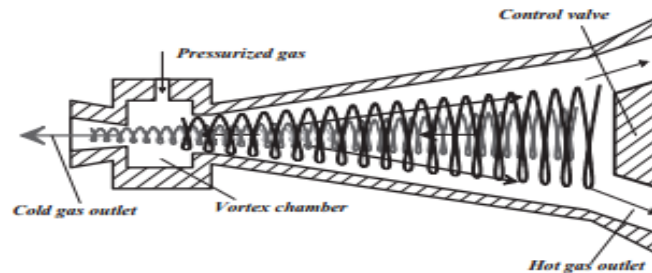
Fig.3 Vortex tube with cylindrical and conical hot tubes
