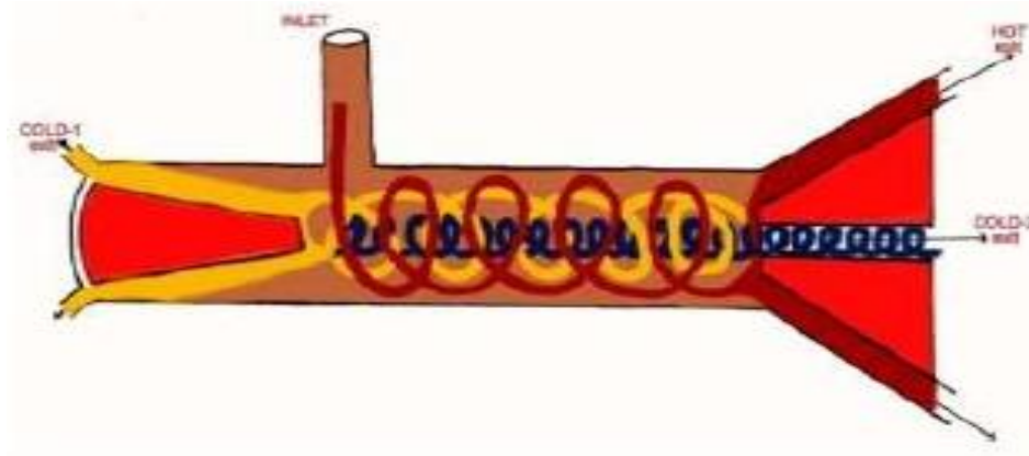
Fig. 5 Flow pattern of the modified vortex tube
