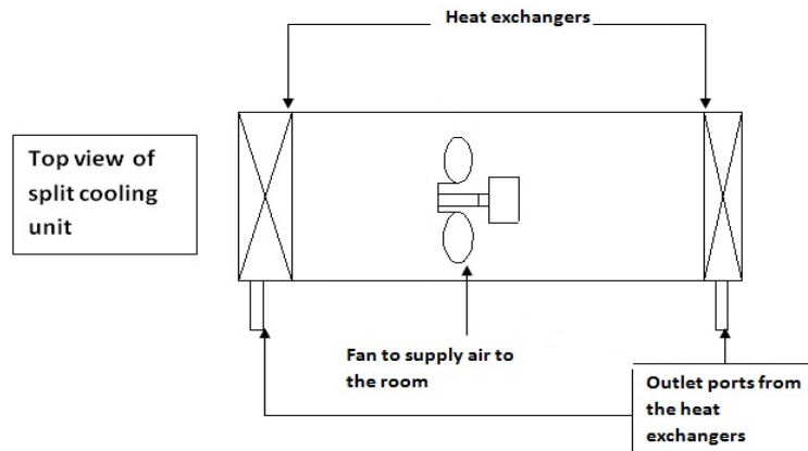
Fig.2 Heat Exchange Mechanism of Split Unit
