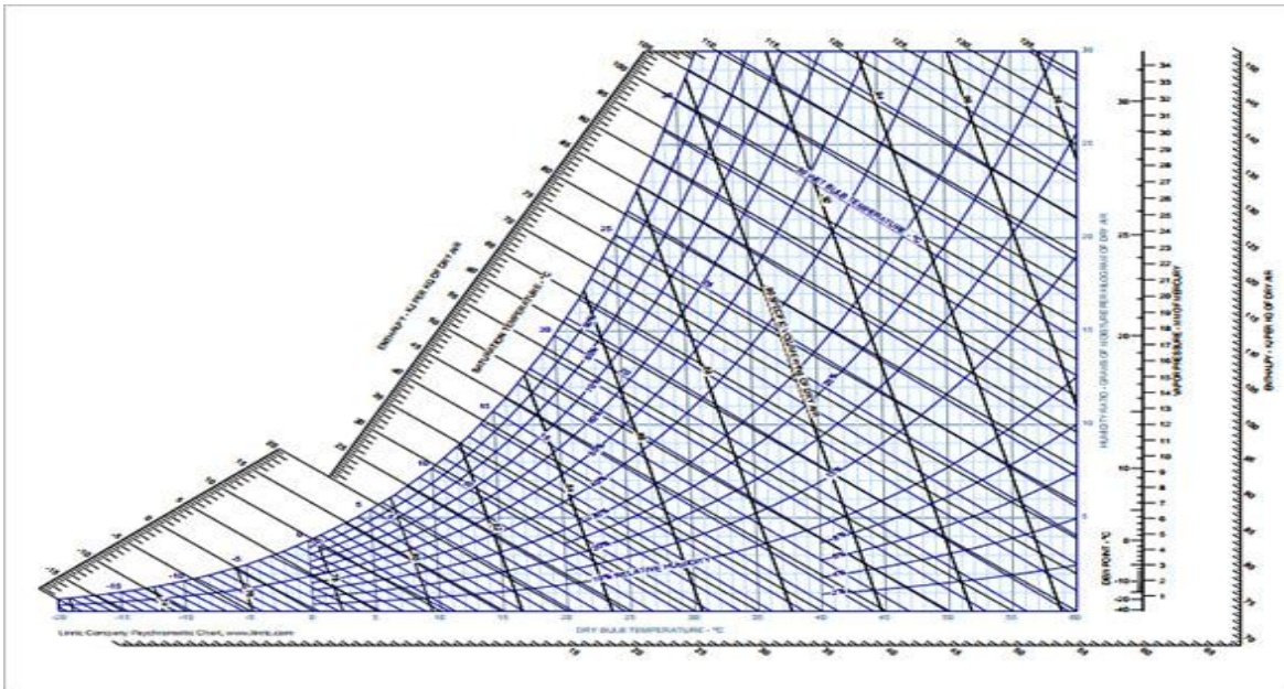
Fig.3 Psychrometric chart showing sensible cooling from 42°C to 23°C while relative humidity remain constant at 50%
