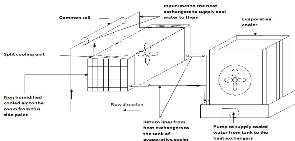
Fig.1 Modified Design of Slip unit
