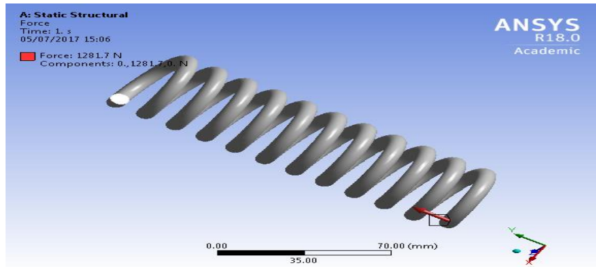
Fig.12 10:3D Modelling of Composite helical spring (Defining Force)
