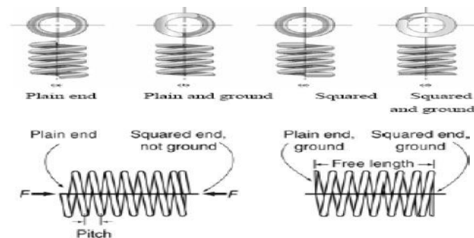
Fig.3 Types of helical spring
