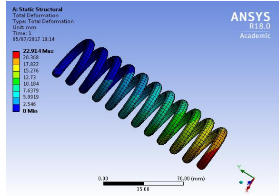
Fig.9 Maximum deflection contour of steel helical spring at 1281.7 N.
