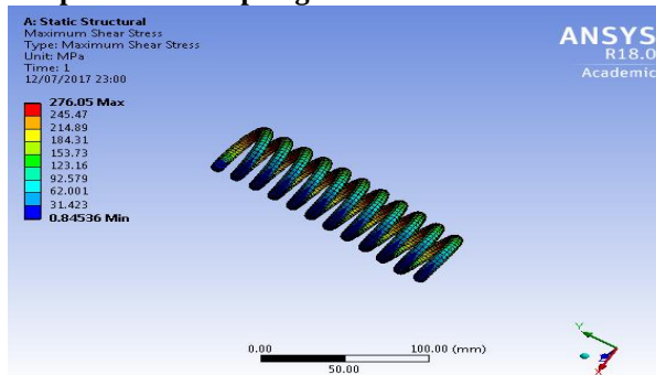
Fig.12 Maximum shear stress contour of composite helical spring at 1281.7 N.
