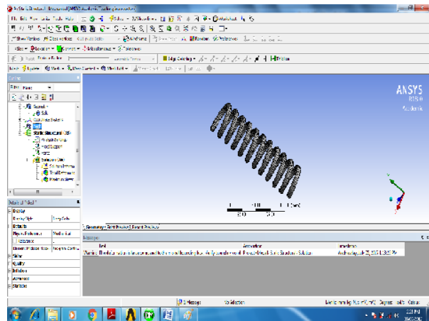
Fig.11 3D Modeling of Composite helical spring (Meshed body)
