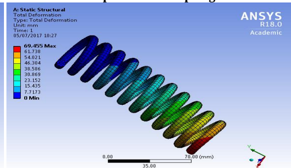
Fig.13 Maximum deflection contour of composite helical spring at 1281.7 N.
