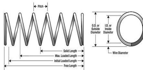
Fig.4 Spring Design
