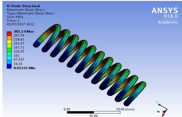
Fig.8 Maximum shear stress contour steel Helical spring at 1281.7 N.
