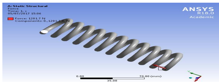
Fig.7 3D Modelling of Steel helical spring (Defining Force)
