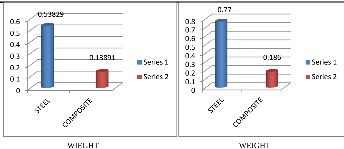
Fig.14: Comparison graph result of weights in steel Helical Spring and composite Helical spring- (a) Analytically (b) Experimentally
