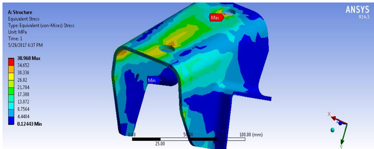
Fig.5 Equivalent (Von-mises) stress contour of Rack and Pinion Assembly Bracket at 1571 N.
