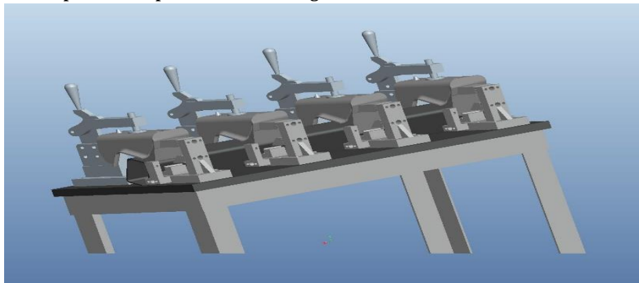
Fig.3 Assembly of Rack and pinion Component with Welding Fixture
