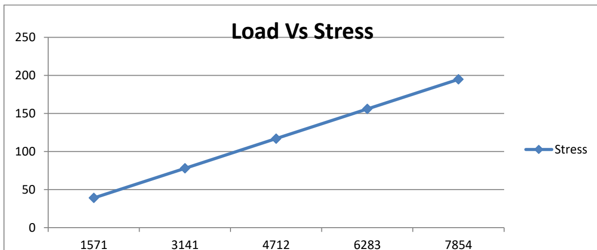
Fig.8 Load Vs stress of rack pinion bracket assembly
