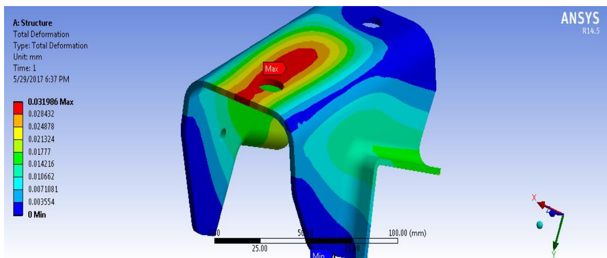
Fig.6 Maximum deflection contour of Rack and Pinion Assembly Bracket at 1571N.
